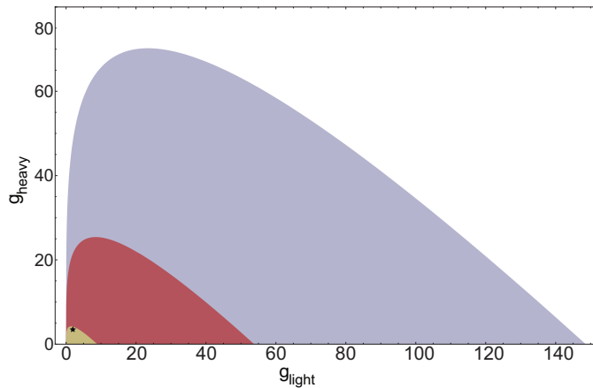
FIG. 1: The allowed values of dark g_{\text{light}} (those degrees of freedom relativistic at T_{\text{BBN}} ) and g_{\text{heavy}} (the remaining dark degrees of freedom) arising from BBN constraints Eqs. (8) and (9). The allowed regions correspond to 95% confidence levels for \xi(T_{\text{RH}}) = 1 and a visible sector g_{* \text{vis}} = 106.75 (red), \xi(T_{\text{RH}}) = 1 and 228.75 (corresponding to MSSM particle content, in blue), and \xi(T_{\text{RH}}) = 1.4(1.7) and g_{* \text{vis}} = 106.75(228.75) (in yellow). The minimal dark sector model of this paper is noted by a black star at g_{\text{light}} = 2 and g_{\text{heavy}} = 3.5 .
