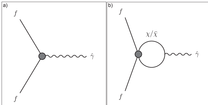
FIG. 5: Feynman diagram leading to \hat{\gamma} interactions with SM fermions f . The vertex in a) can be expanded into that shown in b), as the only particle with an interaction with \hat{\gamma} is the \chi/\bar{\chi} . Since the mass and SU(2)_L charge of these two particles are the same, yet the U(1)_D charges are opposite, the sum of the \chi and \bar{\chi} diagrams in b) is zero, and the overall coupling of f to \hat{\gamma} is therefore zero as well.
