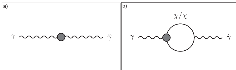
FIG. 4: Feynman diagrams leading to \gamma/\hat{\gamma} mixing. The vertex in a) can be expanded into that shown in b), as the only particle to which the \hat{\gamma} couples is \chi/\bar{\chi} . Since the mass and SU(2)_L charge of these two particles are the same, yet they possess opposite U(1)_D charge, the sum of the \chi and \bar{\chi} diagrams in b) is zero, and the overall mixing vanishes.
