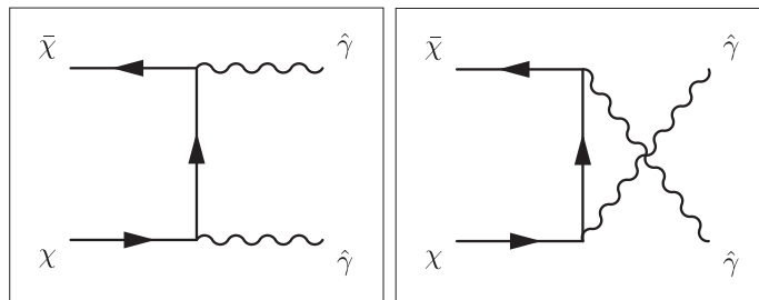
FIG. 2: Pair annihilation/creation of dark matter \chi into dark photons \hat{\gamma} via t and u -channel exchange diagrams. These processes keep the dark sector in thermal equilibrium until the \chi particles become non-relativistic.
